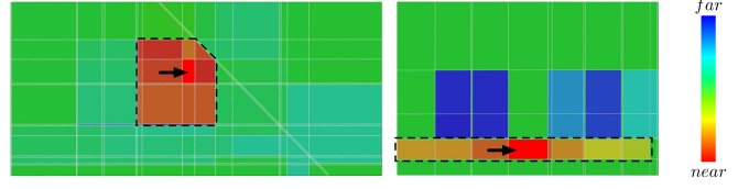
Figure 5: Heatmap visualization of the diffusion distances for two different datasets. In both cases, the distances from a reference face (marked by the arrow) to all other faces in the complex are shown. Note how the cells in the same room (highlighted by the black dotted line) as the source are closer in terms of diffusion distances than the cells that belong to the outer space or to other rooms (shown in green and blue).
