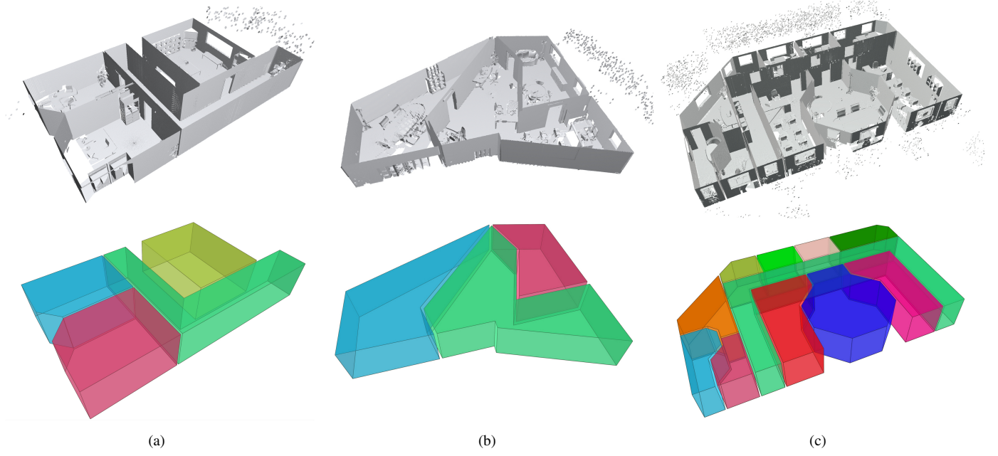
Figure 14: Reconstruction results for the SYNTH 1 (a), SYNTH 2 (b) and SYNTH 3 (c) datasets. It can be seen how our algorithm can successfully deal with environments that do not satisfy the Manhattan-World assumptions and that contain rooms with complex and irregular boundaries. Notice the presence of scattered points outside of the windows, added to the virtual scans to simulate the artifacts from laser rays hitting reflective surfaces (e.g. glass). As in Fig. 13 we have removed the top part of the input model for the sake of clarity.
