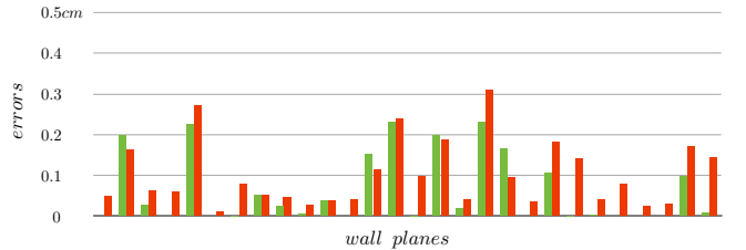
Figure 11: Accuracy of the final wall planes reconstruction using the new IRLS method (green) and the LMS method (red). The plots refers to dataset SYNTH 1. For each wall plane of the reconstructed model (on the horizontal axis) the maximum distance from the plane to the set of points used for the fit is shown. The accuracy of IRLS is comparable and generally better than the one obtained using LMS.
