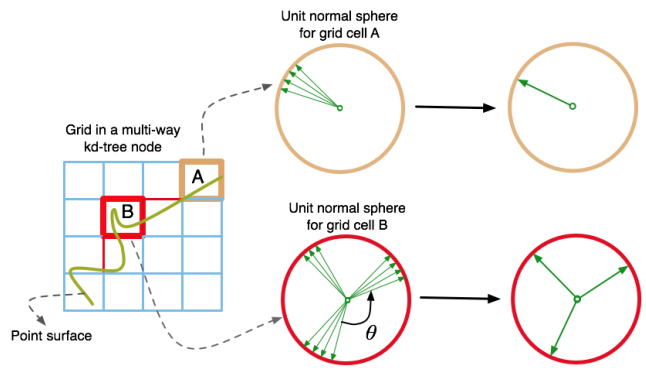
Fig. 3 Normal deviation clustering. Points (shown by green arrows in their unit normal spheres) within a grid cell are clustered according to their normal deviation.
