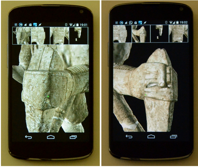
Figure 4: Detail of model interactively rendered on a Nexus 4 smartphone. This 70Mtriangles model is colored using post-restoration color data. Note how our compression preserves extremely high quality details in shape, normal, and colors.
