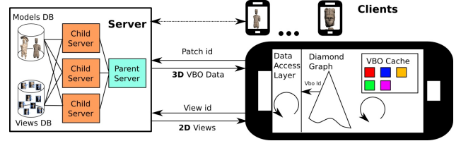
Figure 3: Client-server architecture.
