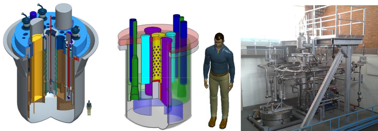
Figure 4. The MYRRHA reactor and the scaled down ESCAPE facility (SCK•CEN).
