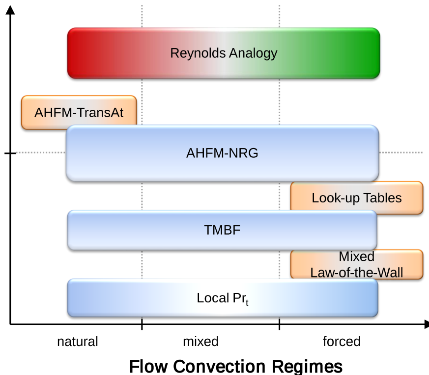
Figure 1. Liquid metal models identified in [15, 16] and their applicability for different fluids and different flow regimes. The models indicated in blue will be further developed and tested in the SESAME and MYRTE projects.
