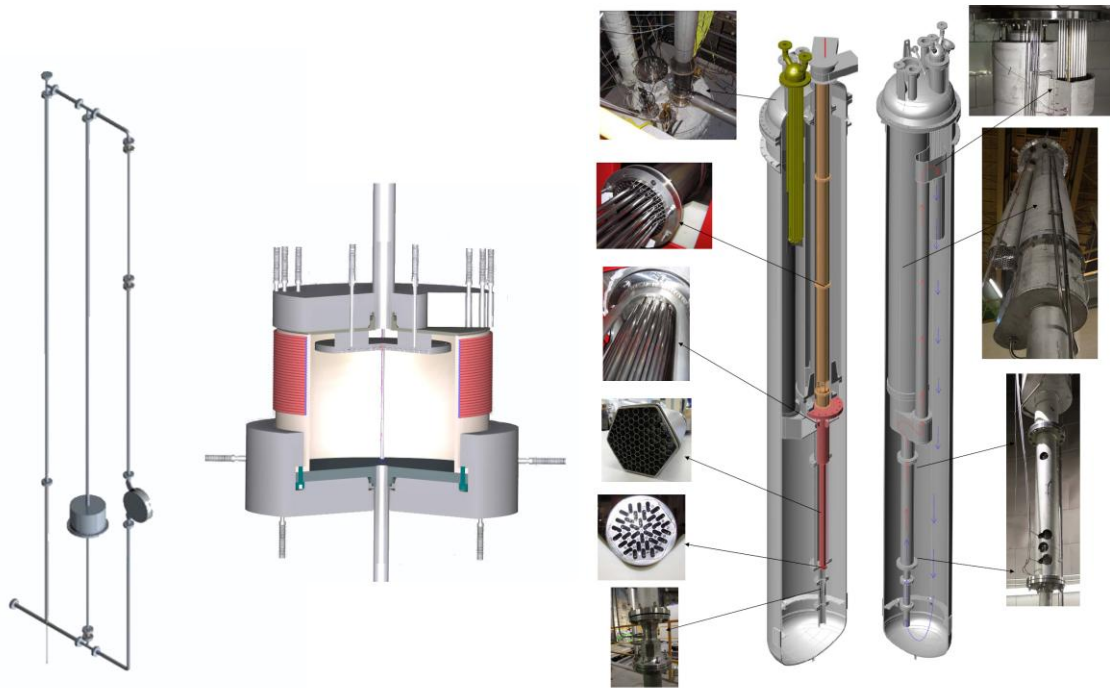
Figure 5. Loop and 3-dimensional test section of the TALL-3D loop (left) and an overview of the CIRCE test section (right).
