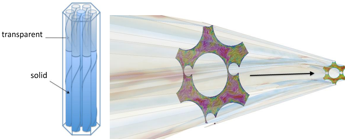
Figure 2. Sketch of a 7 pin wire wrapped bundle MIR experiment (TUD) and instantaneous snapshot of initial test simulation to obtain high fidelity numerical reference data for an infinite pin bundle (NRG).
